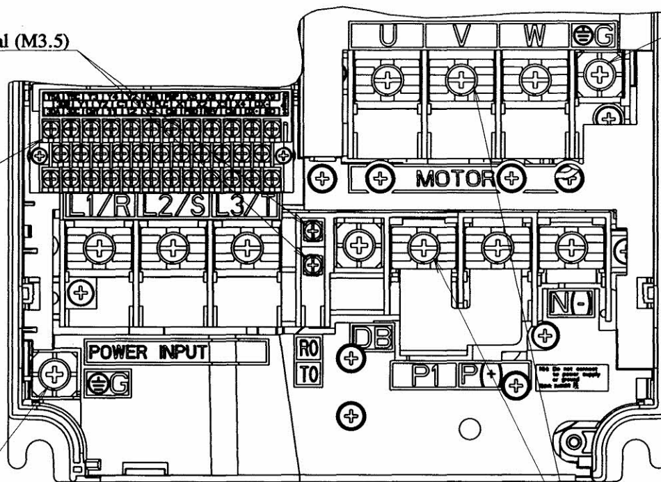
Terminal location 端子配置 Scale 1:2
